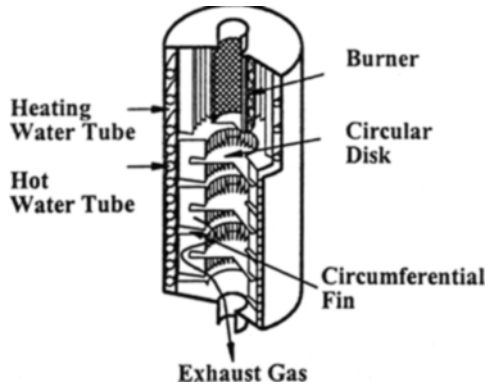
Fig. 1 Heat exchanger suggested for a condensing boiler
