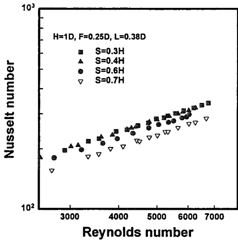
Fig. 10 The effect of the fin-disk spacing on the Nusselt number
